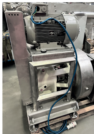
Indirect motorization
