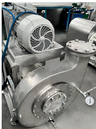
Indirect motorization
