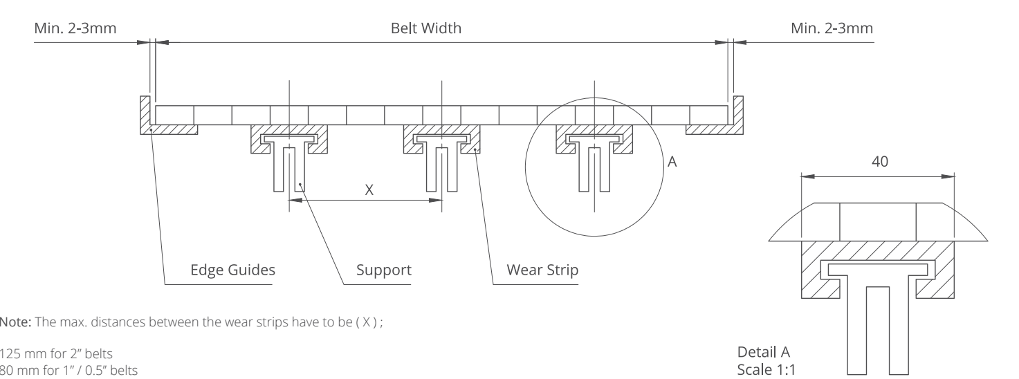
HP508 Series / Slider Support System For Straight Running Belts
